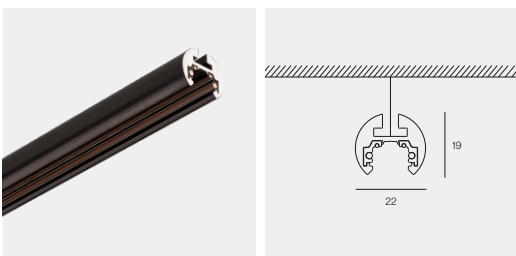
XS Track M19O Suspended 016
