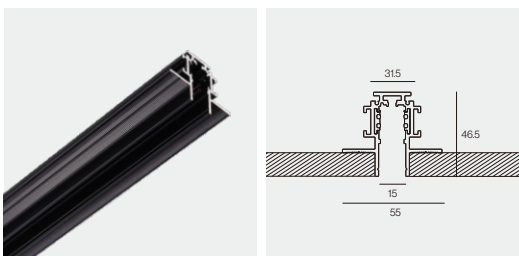
Slim Track M15E Trimless Recessed 068
