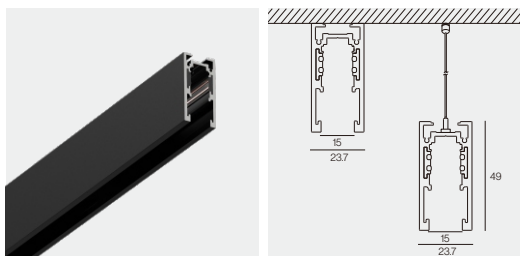
Slim Track M15A Surface/Suspended 067
