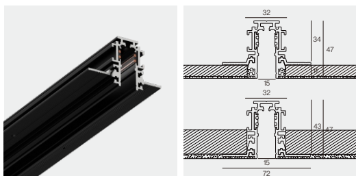
Slim Track M15F Trimless 069
