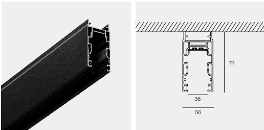
Motorized M56A Surface Mounted 159
