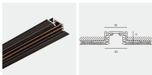
XS Track M19T Trimless Recessed 017
