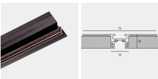
XS Track M19E Trimless Recessed 018
