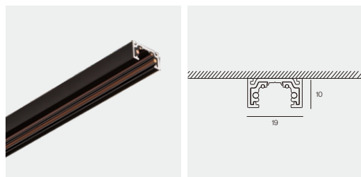
XS Track M19A Surface 015
